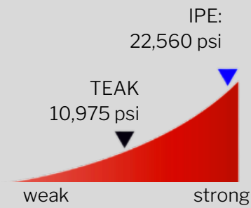
Ipe Bending Strength
